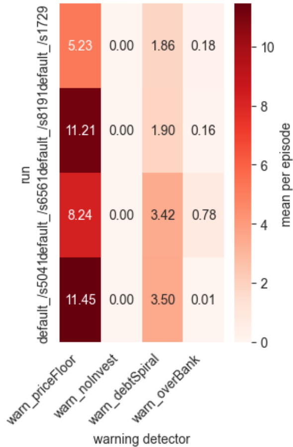
Mean warning-flag counts per episode in the converged window (last 200 eps)
